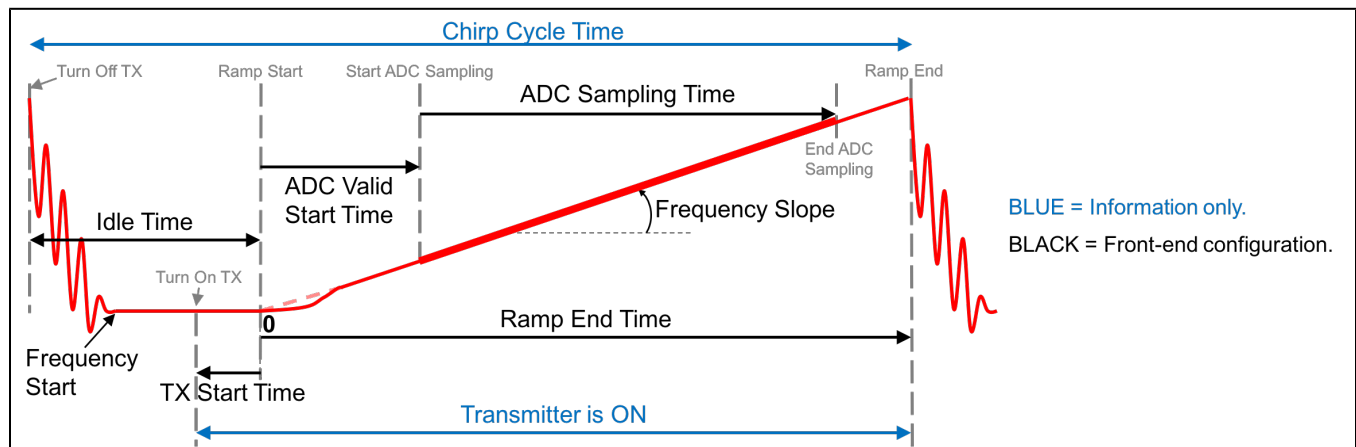
Figure 2: Chirp Diagram
