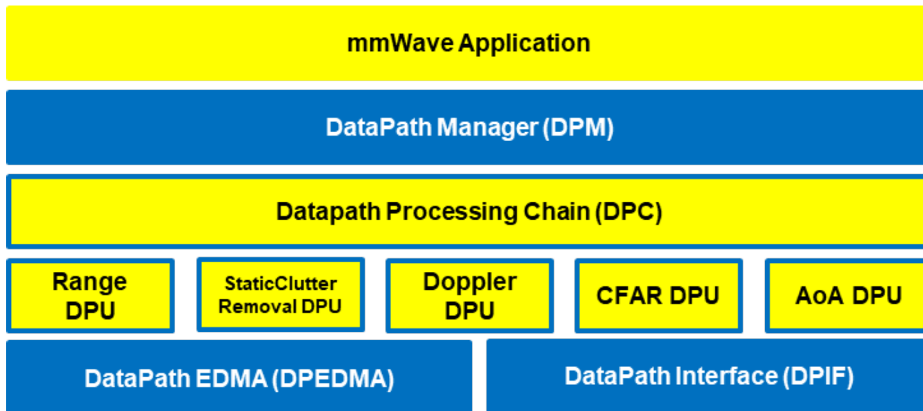
Figure 18: Typical mmWave Detection Processing Layers
