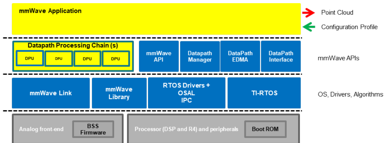
Figure 7: SDK Layered block diagram
