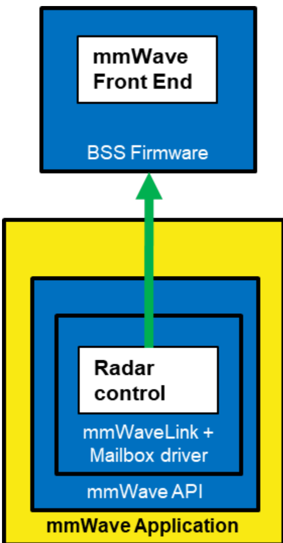
Figure 11: Typical mmWave radar control flow
