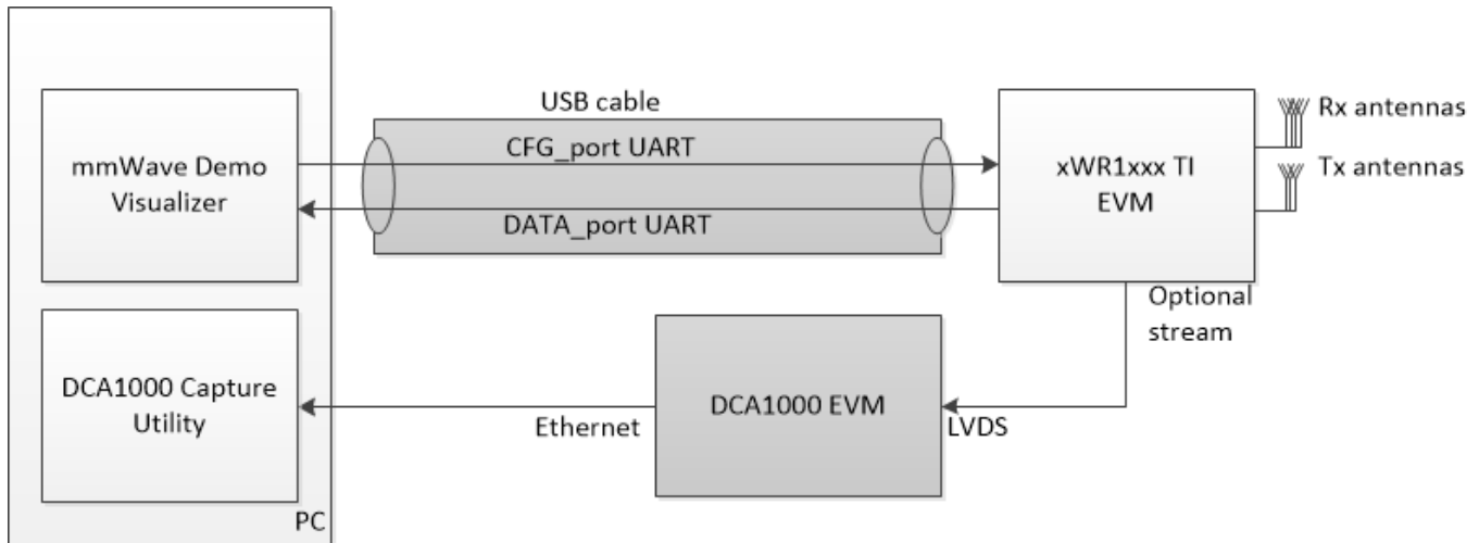
3. 3. 1. 0. 1Figure 1: mmWave Demo Visualizer- mmWave Device Connectivity
