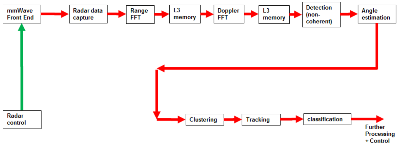
5. 2. 0. 0. 1Figure 8: Typical mmWave radar processing chain
