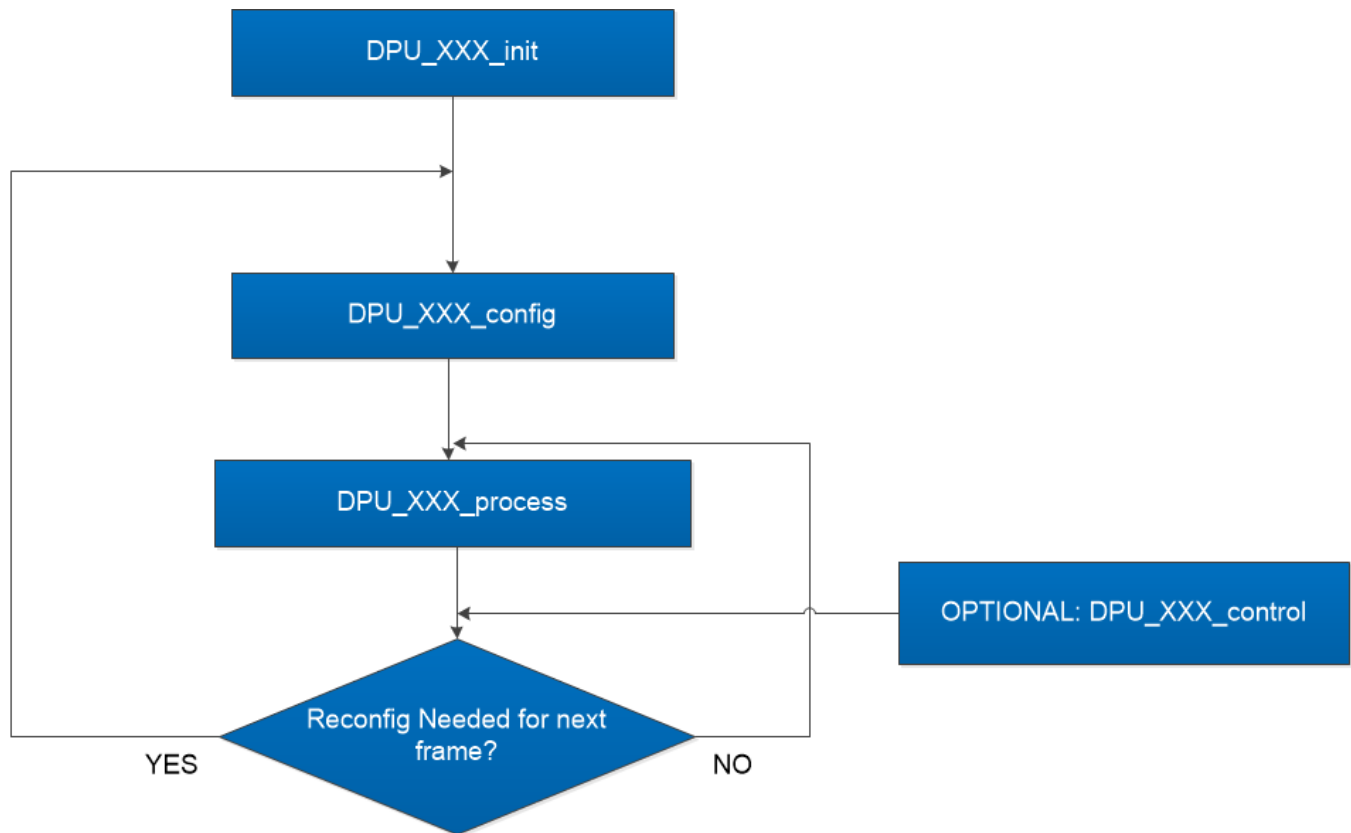
5. 4. 7. 0. 4Figure 31: DPU - typical call flow
