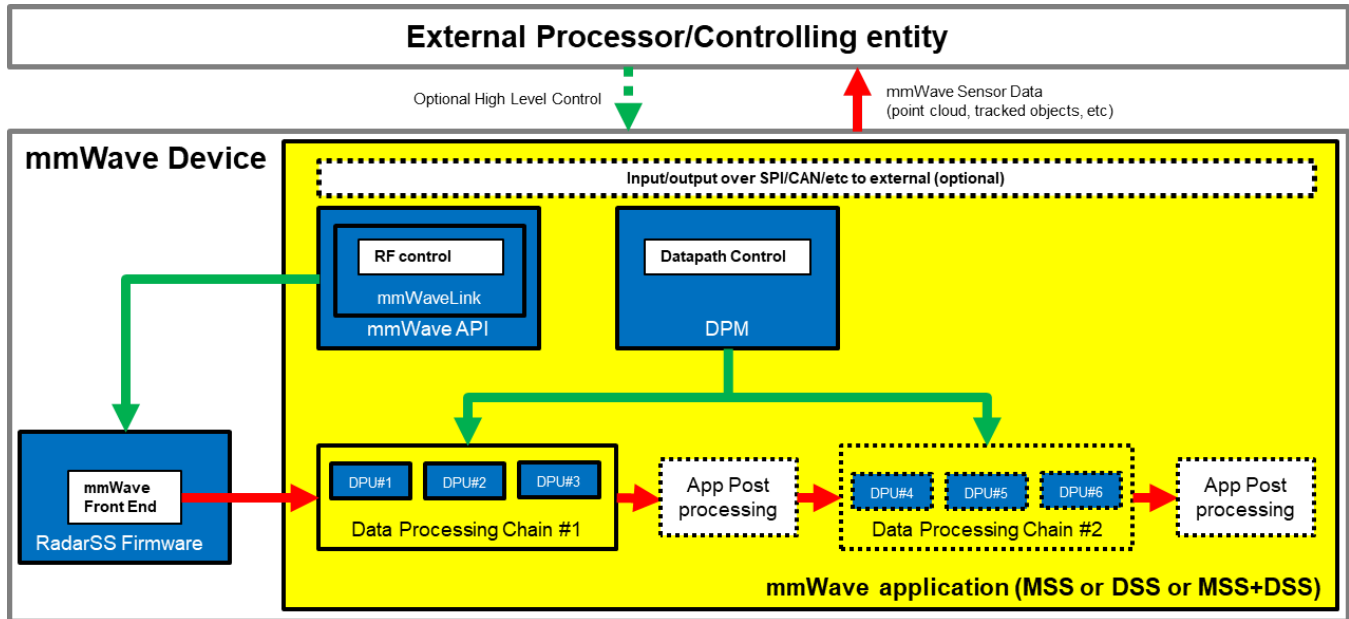
5. 1. 0. 0. 1Figure 6: Autonomous mmWave sensor (Standalone mode)
