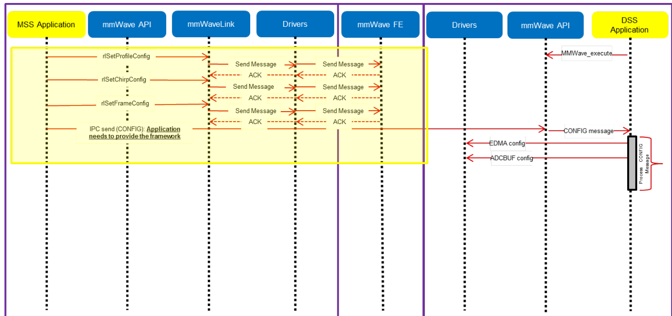
5. 4. 5. 2. 1Figure 28: mmWave API - 'Minimal' Config - Sample flow (mmWave devices with MSS and DSS cores and module in co-operative mode)
