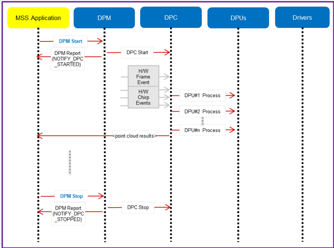
5. 3. 2. 1. 2Figure 20: Data processing flow with local domain control (start/chirp/frame/stop)
