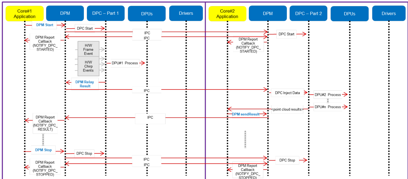
5. 3. 2. 3. 2Figure 24: Distributed Data processing flow and control (start/chirp/frame/stop)
