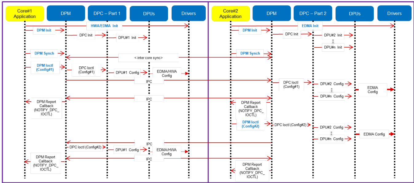
5. 3. 2. 3. 1Figure 23: Distributed Data processing flow and control (init/config)
