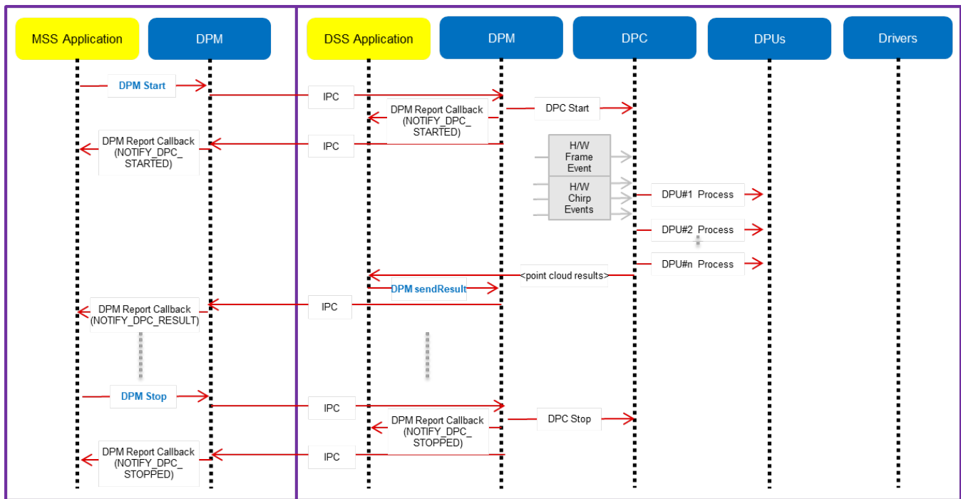
5. 3. 2. 2. 2Figure 22: Data processing flow with remote domain control (start/chirp/frame/stop)
