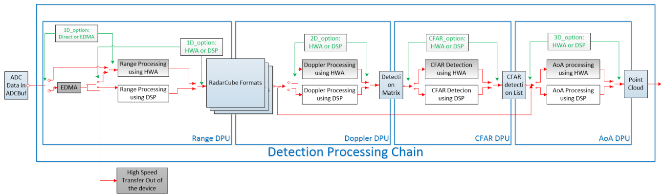
5. 2. 0. 0. 1Figure 10: Scalable data processing chain using mmWave SDK
