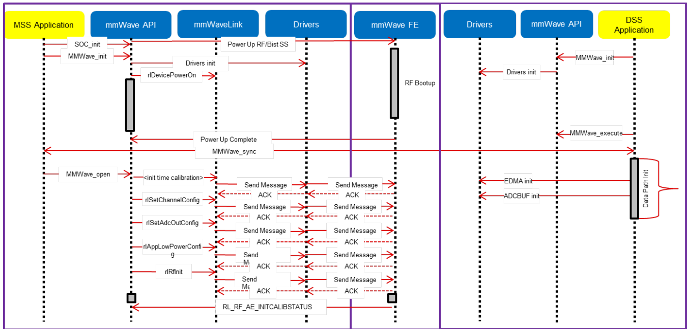
5. 3. 1. 2. 1 Figure 15: mmWave Co-operative Mode: Detailed Control Flow (Init sequence)
