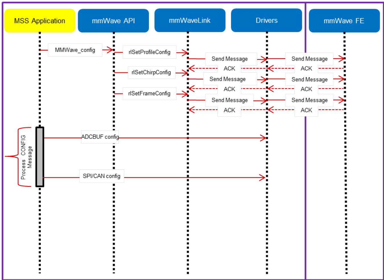
5. 3. 1. 1. 2Figure 13: mmWave Isolation mode: Detailed Control Flow (Config sequence)
