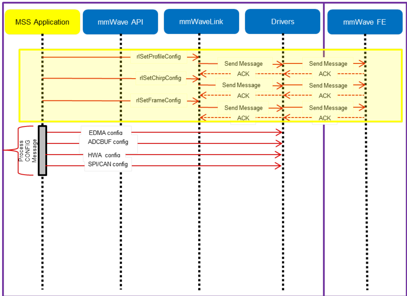
5. 4. 5. 2. 2Figure 29: mmWave API - 'Minimal' Config - Sample flow (mmWave devices with single core or when module is used in isolation mode)
