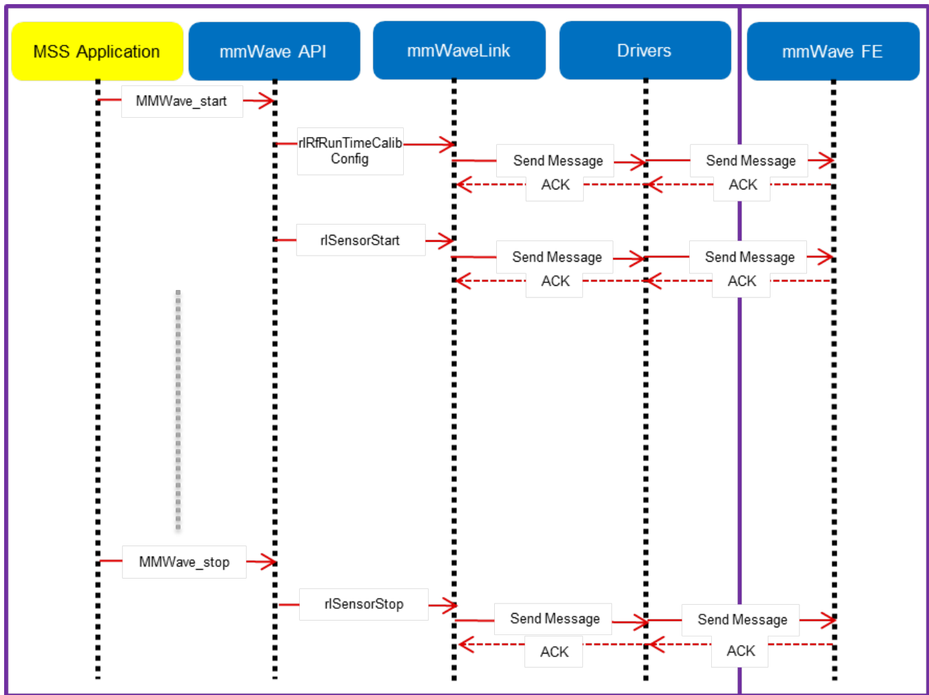
5. 3. 1. 1. 3Figure 14: mmWave Isolation mode: Detailed Control Flow (start sequence)
