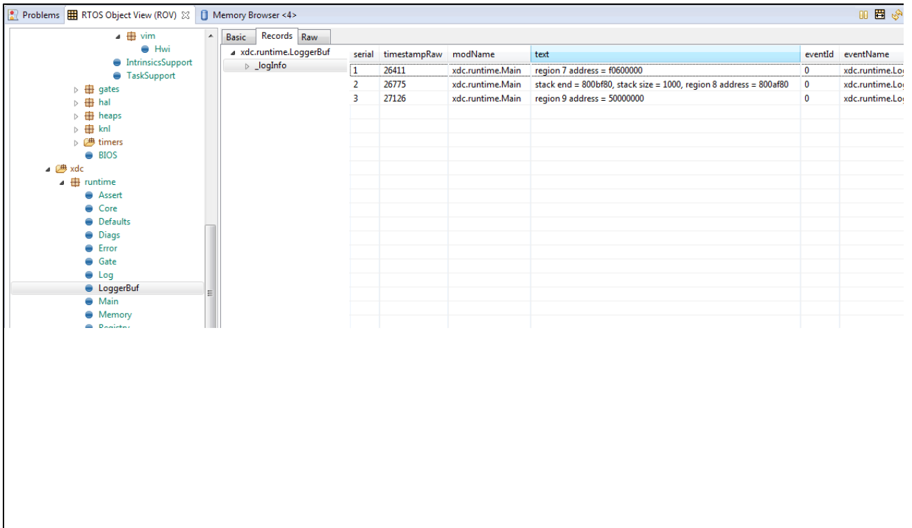
6. 3. 0. 0. 1 Figure 33: Sample ROV log with debug prints
