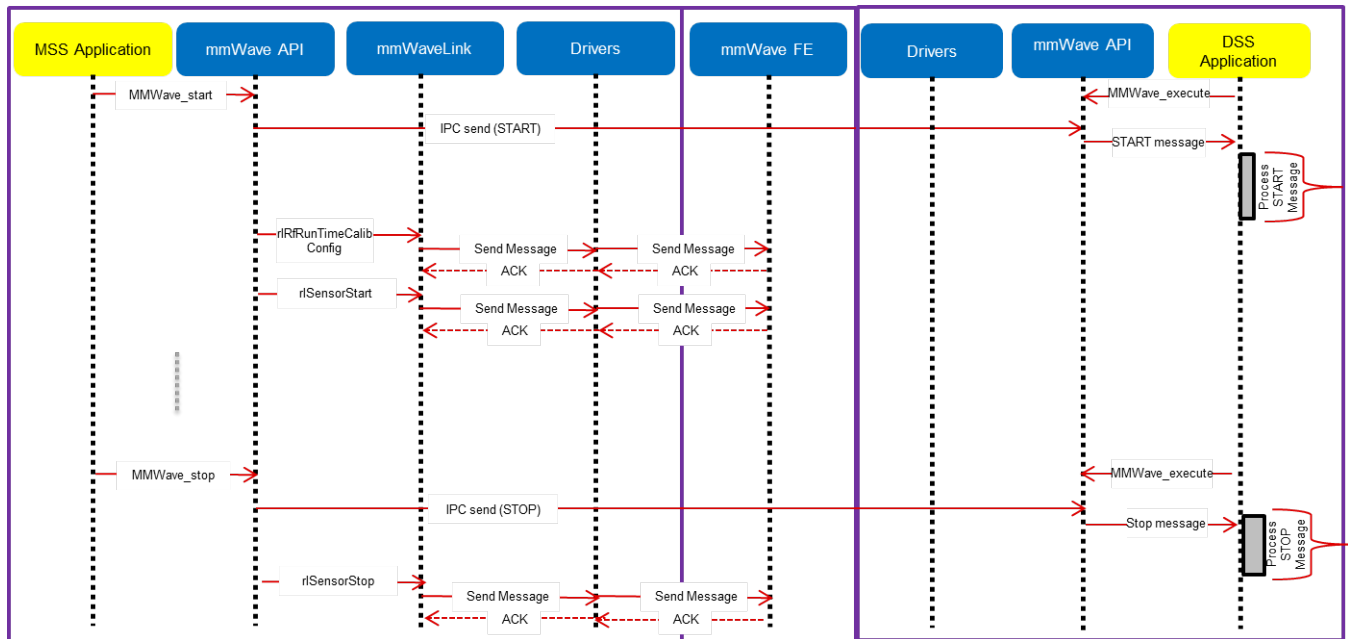
5. 3. 1. 2. 3Figure 17: mmWave Co-operative Mode: Detailed Control Flow (Start sequence)
