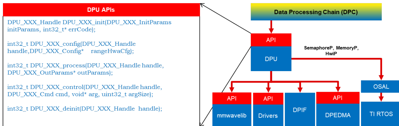
5. 4. 7. 0. 3Figure 30: DPU - Internal software design
