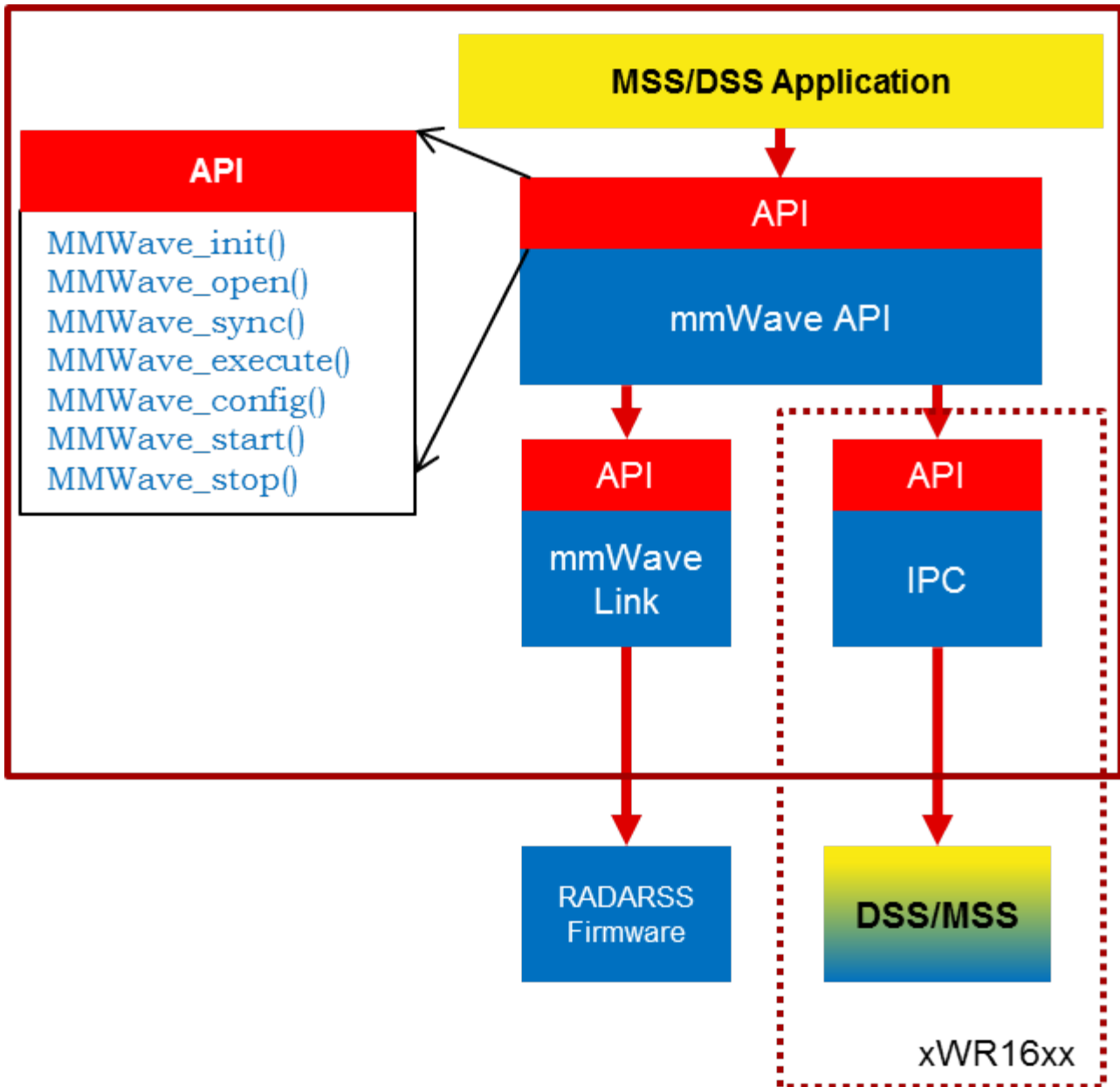
5. 4. 5. 0. 4Figure 27: mmWave API - Internal software design
