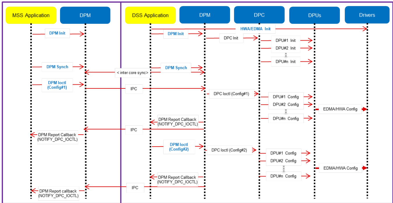
5. 3. 2. 2. 1Figure 21: Data processing flow with remote domain control (init/config)
