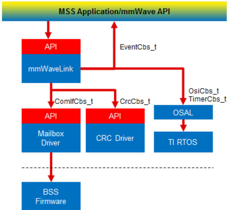
5. 4. 4. 0. 3Figure 26: mmWaveLink - Internal software design
