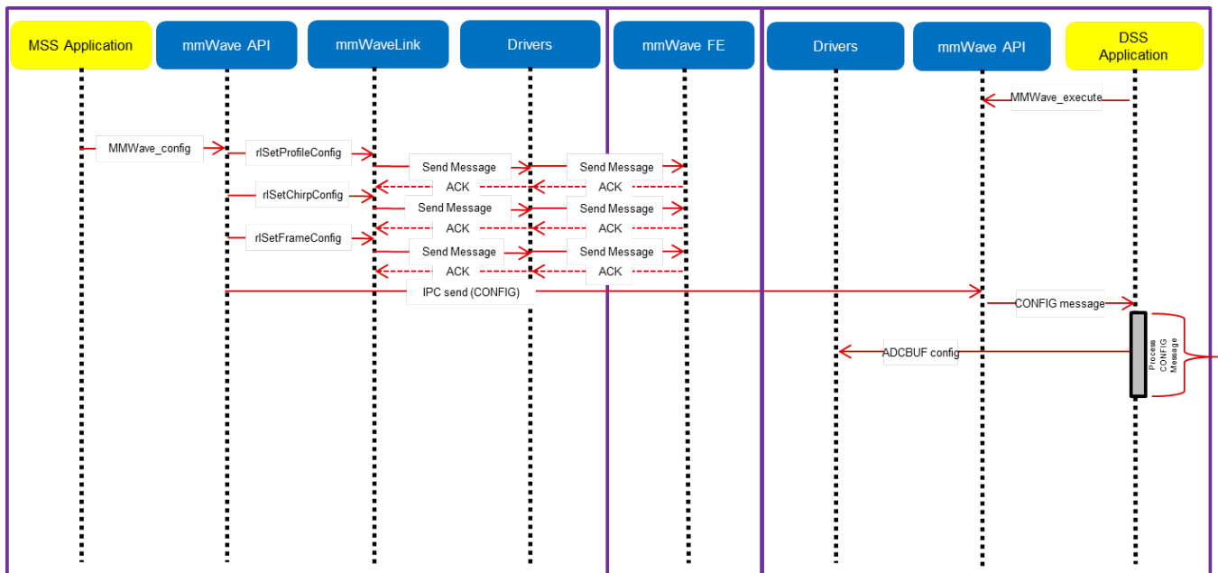
5. 3. 1. 2. 2 Figure 16: mmWave Co-operative Mode: Detailed Control Flow (Config sequence)
