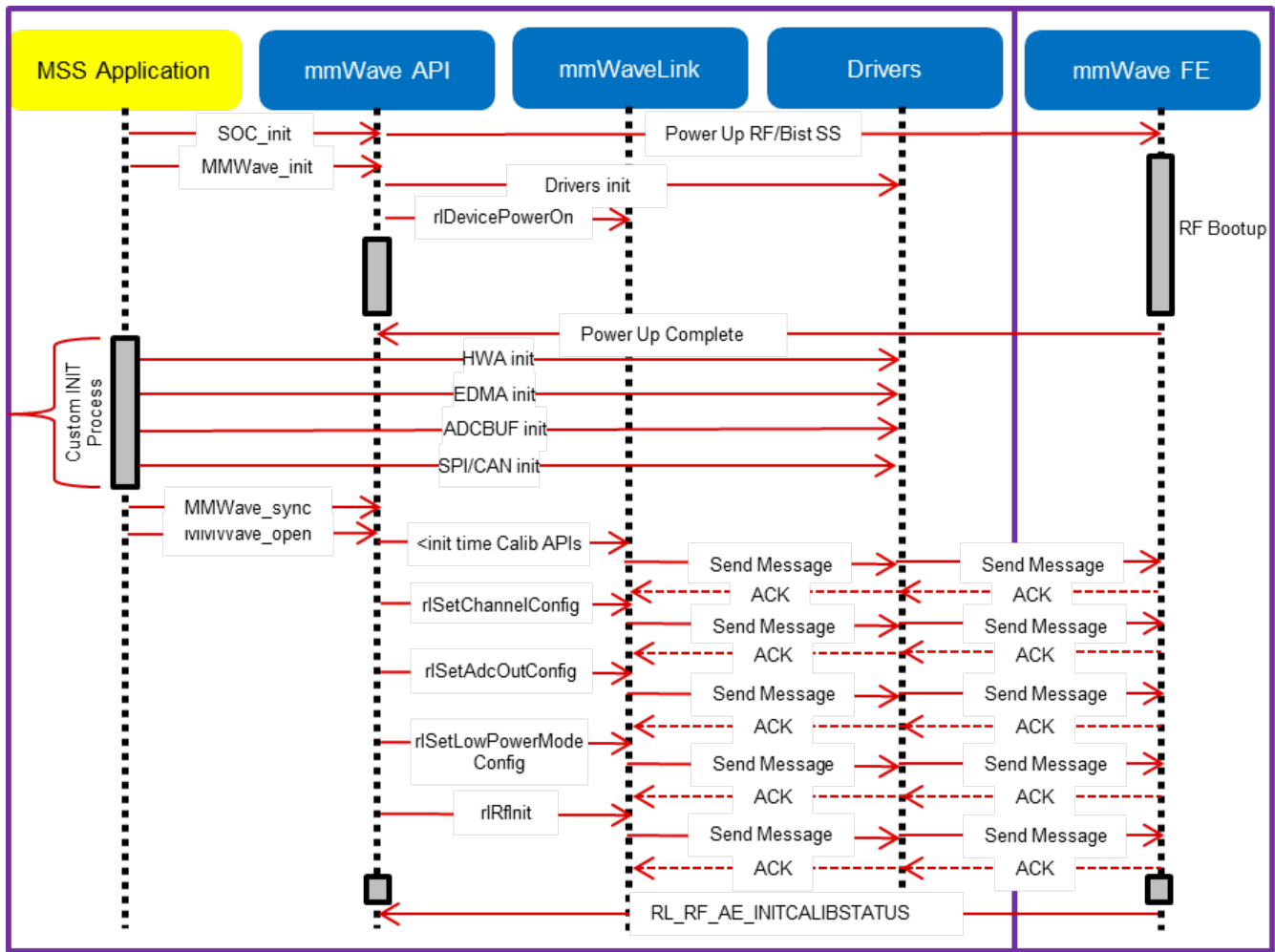
5. 3. 1. 1. 1Figure 12: mmWave Isolation mode: Detailed Control Flow (Init sequence)
