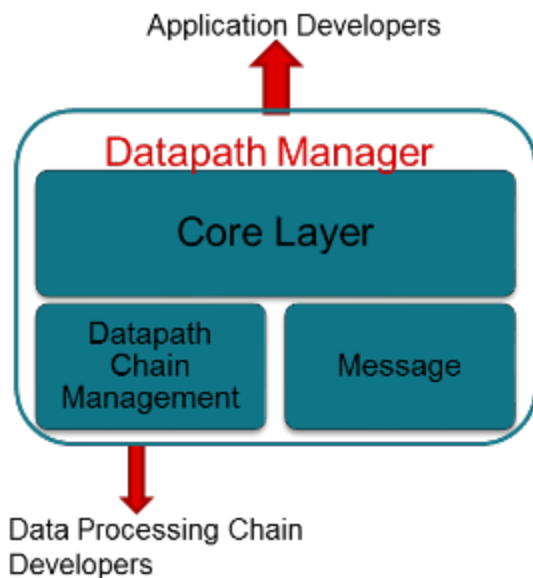
5. 4. 8. 0. 5Figure 32: Datapath manager (DPM) - internal software design
