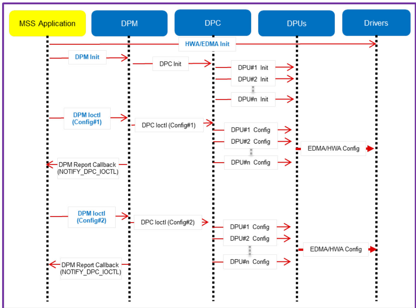
5. 3. 2. 1. Figure 19: Data processing flow with local domain control (init/config)
