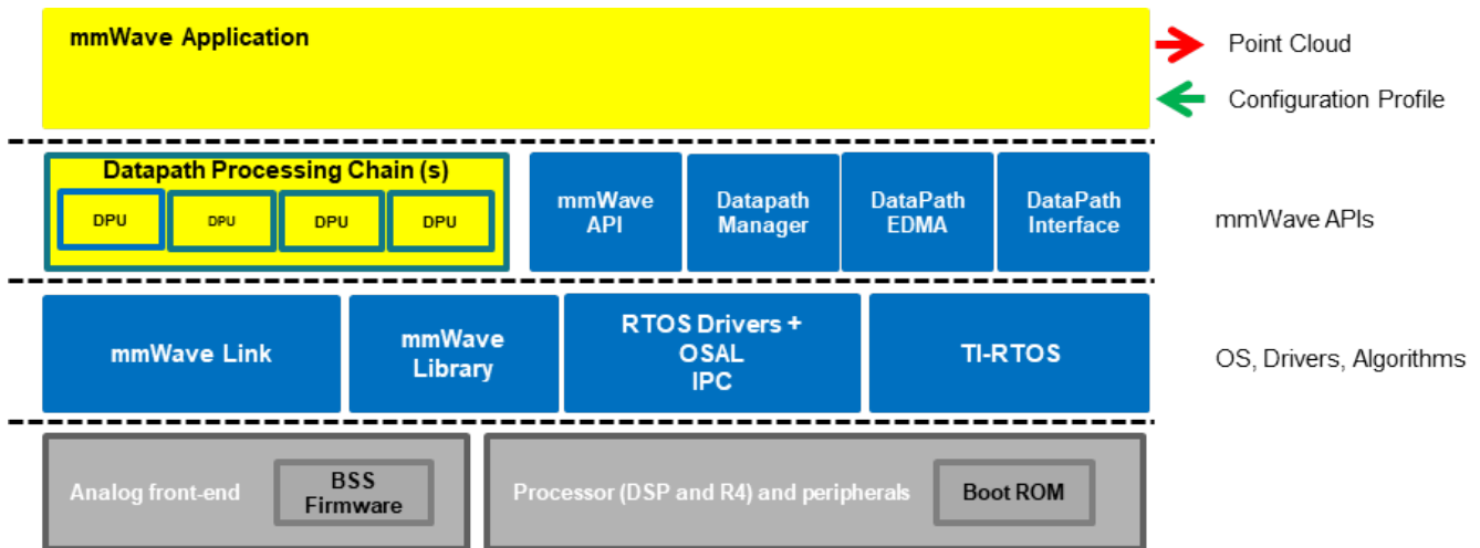
5. 1. 0. 0. 1Figure 7: SDK Layered block diagram
