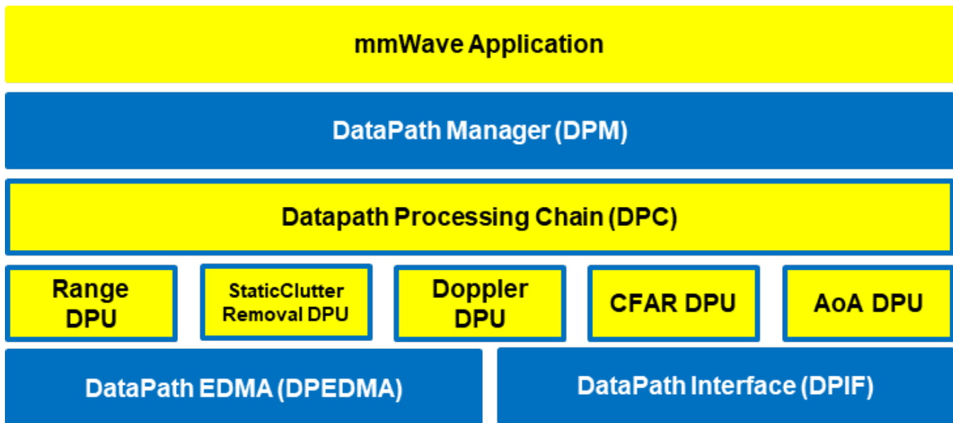
5. 3. 2. 0. 4Figure 18: Typical mmWave Detection Processing Layers
