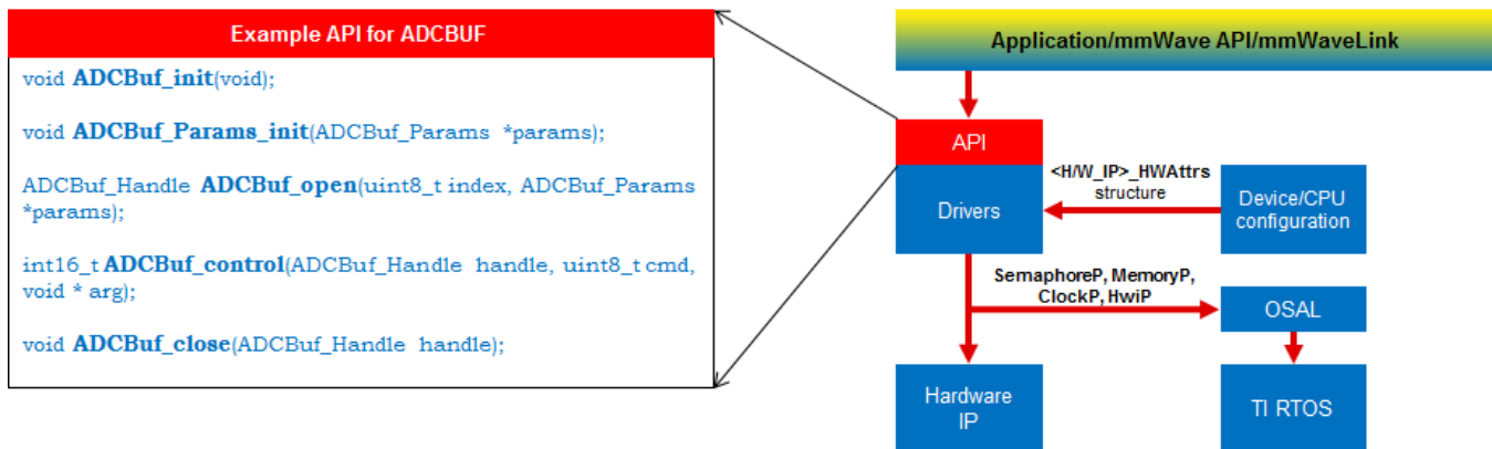
5. 4. 2. 0. 1Figure 25: mmWave SDK Drivers - Internal software design
