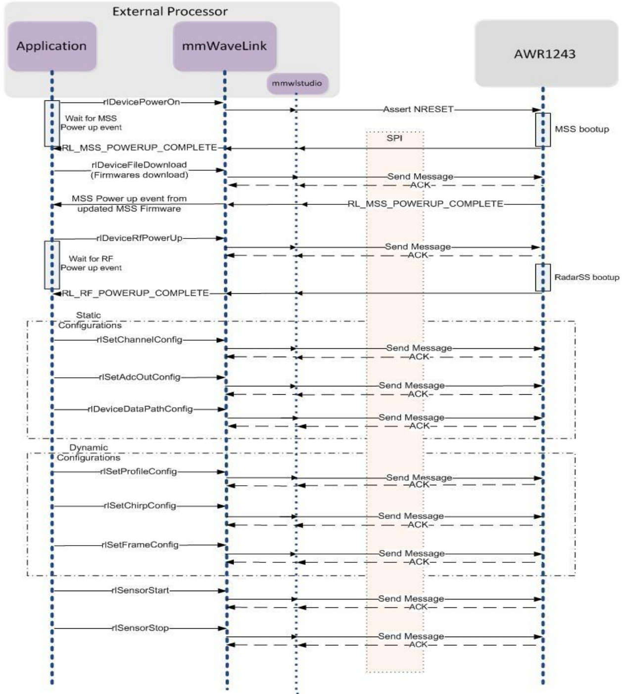
Figure 13. API Sequence
